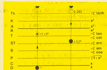
Abb. 68 \varphi = 17,13^\circ
