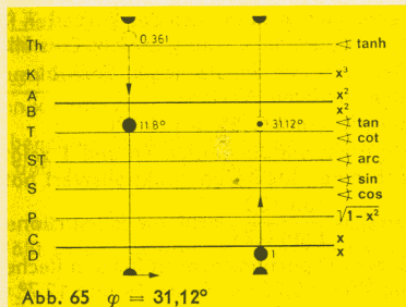
Abb. 65 \varphi = 31,12^\circ
