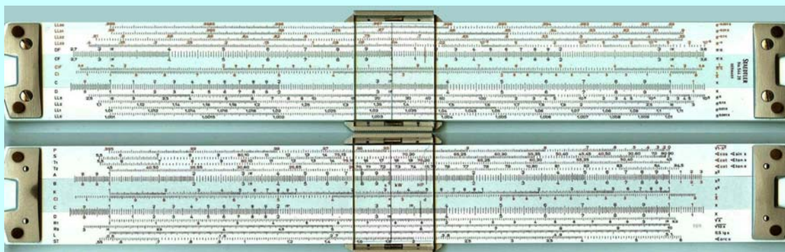
STAEDTLER 544-28 LOG LOG
